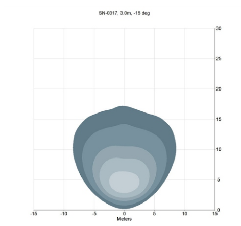
1015 - 2250 Wide 45°+ Symmetrical
