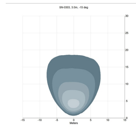
1015 - 2250 Wide 45°+ Asymmetrical
