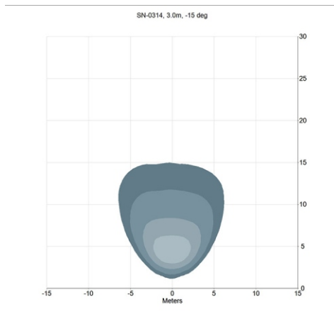
1015 - 1450 Wide 45°+ Symmetrical
