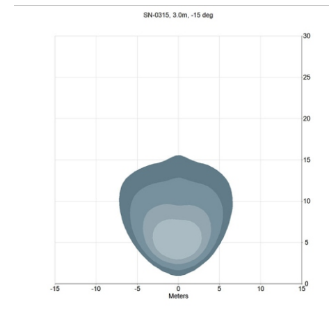
1015 - 1450 Wide 45°+ Asymmetrical
